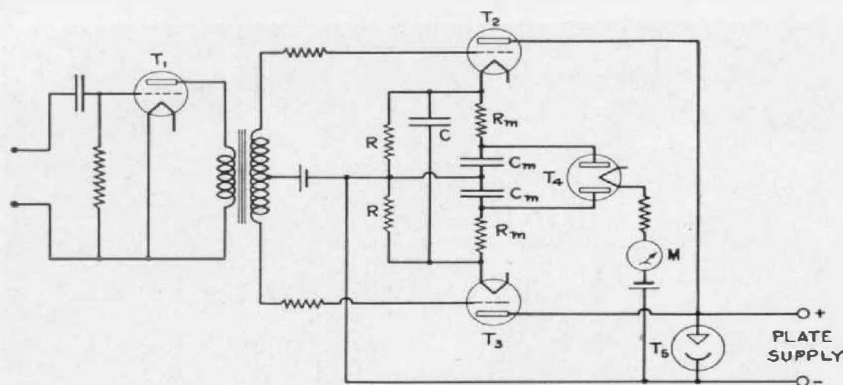
FIGURE 1. Schematic circuit diagram of the electronic frequency meter. For convenience, batteries are shown supplying the grid and meter biases. T_1 is an amplifier, T_2 and T_3 are gas-discharge tubes; T_4 is a double diode, and T_5 a voltage regulator. The circuits R , C , control the voltage on the grids of the gas-discharge tubes; the circuits R_m , C_m , control the action of the double diode
