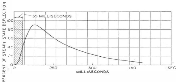
FIGURE 1 (left). Plot of meter deflection vs. time when a pulse of 55 milliseconds duration is applied. The pulse length is just sufficient to bring the meter to 90% of its steady-state reading on a pulse of the same amplitude. Note that the meter does not reach its maximum deflection until after the end of the pulse
